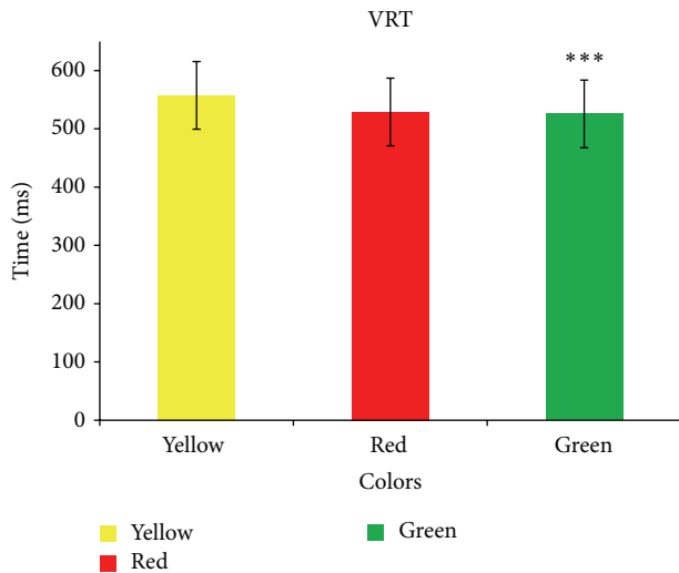
FIGURE 1: Comparison of visual choice reaction time among colors. Values are expressed as mean \pm SD; analysis was done by repeated measures ANOVA. * P < 0.05 ; ** P < 0.01 ; *** P < 0.001 . F value, 15.01. VRT: visual reaction time.
